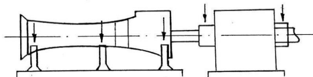
Fig. 9.8.1 Points of vibration measuring (the points and directions of vibration measurement are shown by arrows)
