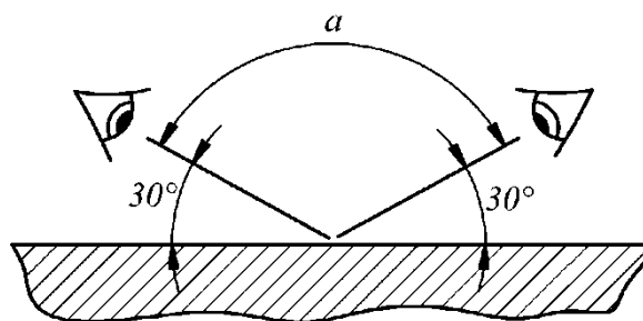
Fig. 3.2.2.5 Access conditions to check surface at visual and measurement testing
