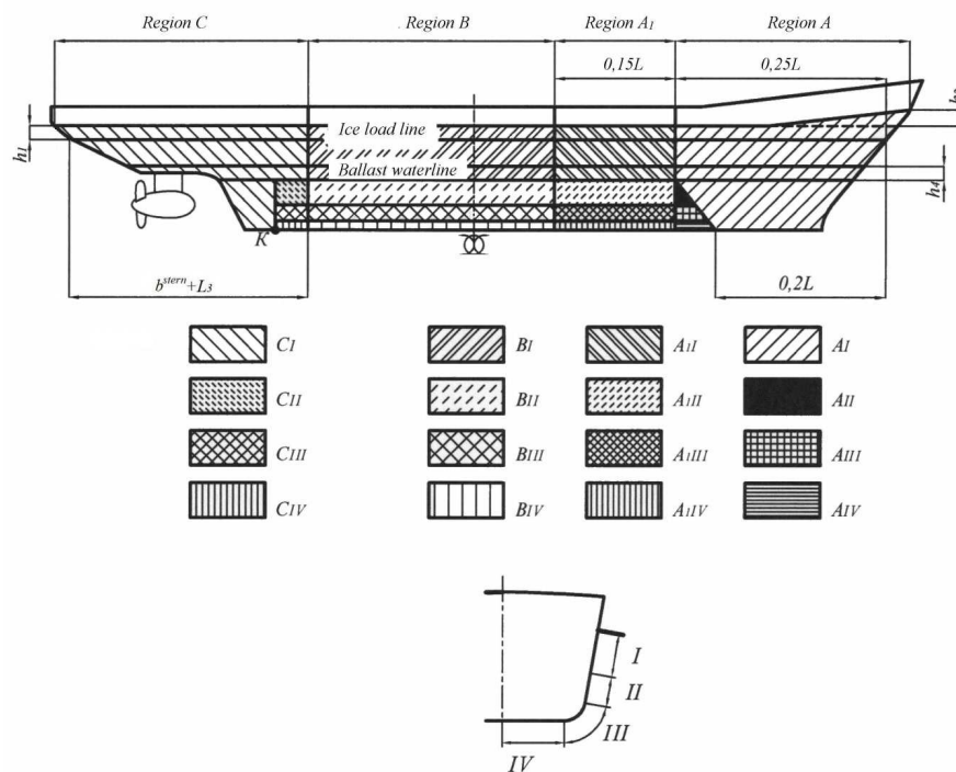
Fig. 19.2.2.4 Regions of ice strengthening of Arctic double acting ships with ice class mark Icebreaker6 or Icebreaker7 in the class notation when operating stern first: b^{stern} = distance from the point of the ice load line and sternframe intersection to the section where the ice load line is the widest, but not greater than 0,2L
