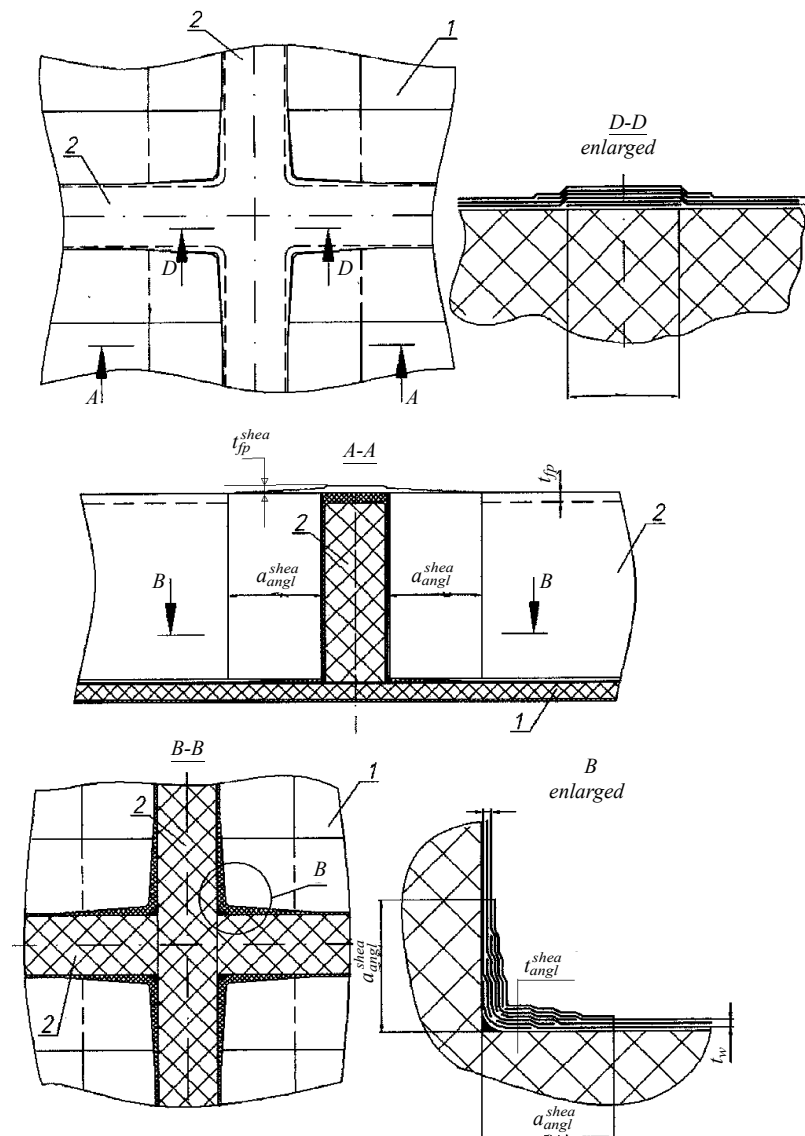
Fig. 3.20 Intersection of the longitudinal and intercostal transverse framing members of similar depths, with continuous face plates: 1 — shell (deck); 2 — framing members (scantlings of matted-on sheathings shall be determined according to the following formula: t_{fp}^{shea} \cong t_{fp} ; t_{angl}^{shea} \cong t_w ; a_{angl}^{shea} \geq 12t_{angl}^{shea}
