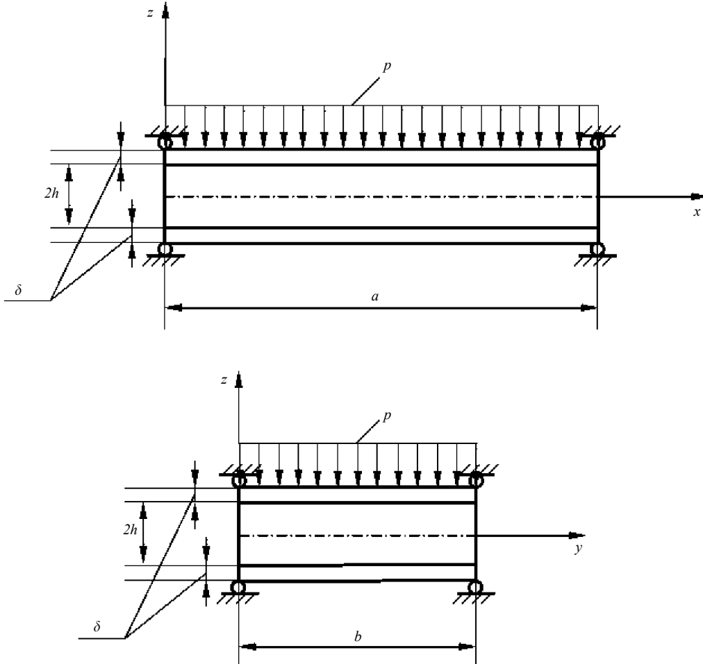
Fig. 9 Load type of the sandwich plate
