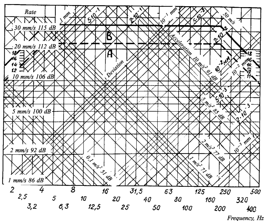
Fig. 9.3.4 Vibration standards for turbo-compressors of internal combustion engines:
