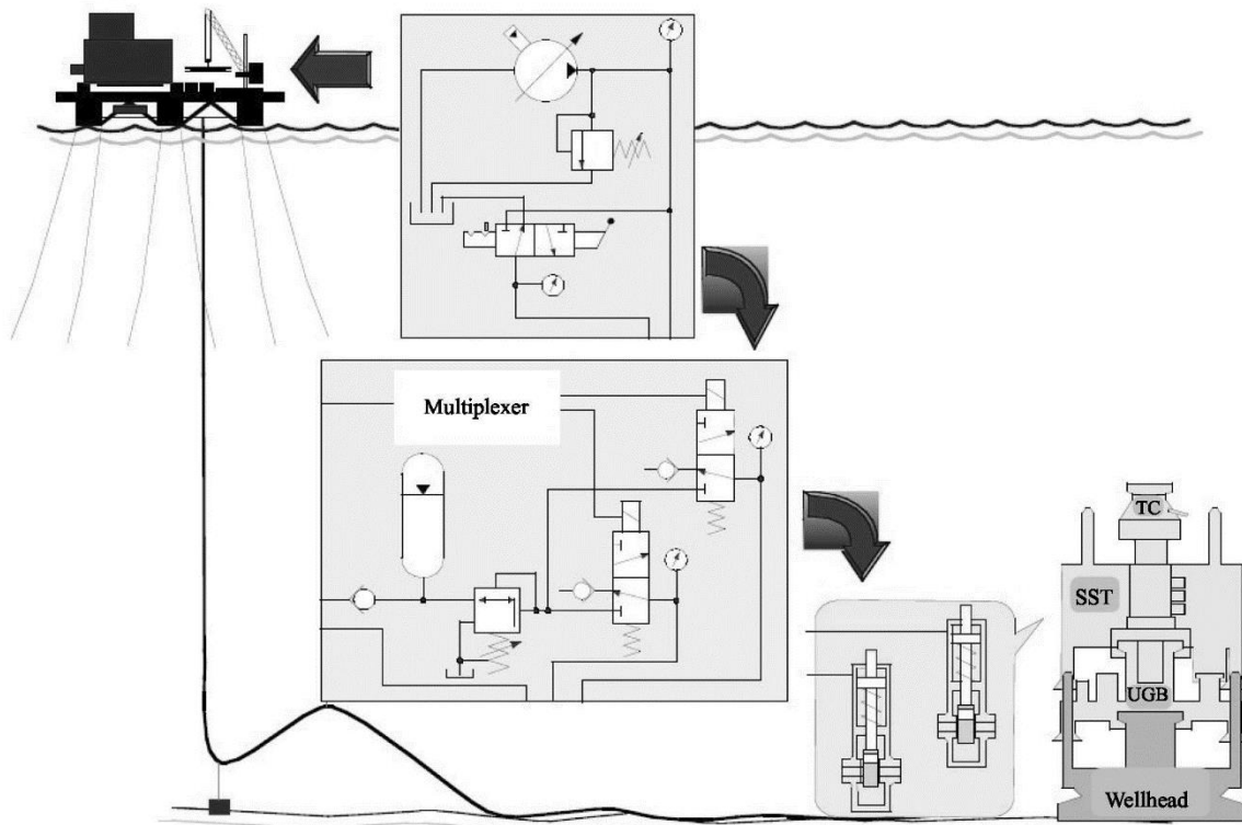
Fig. 6 Multiplex systems
