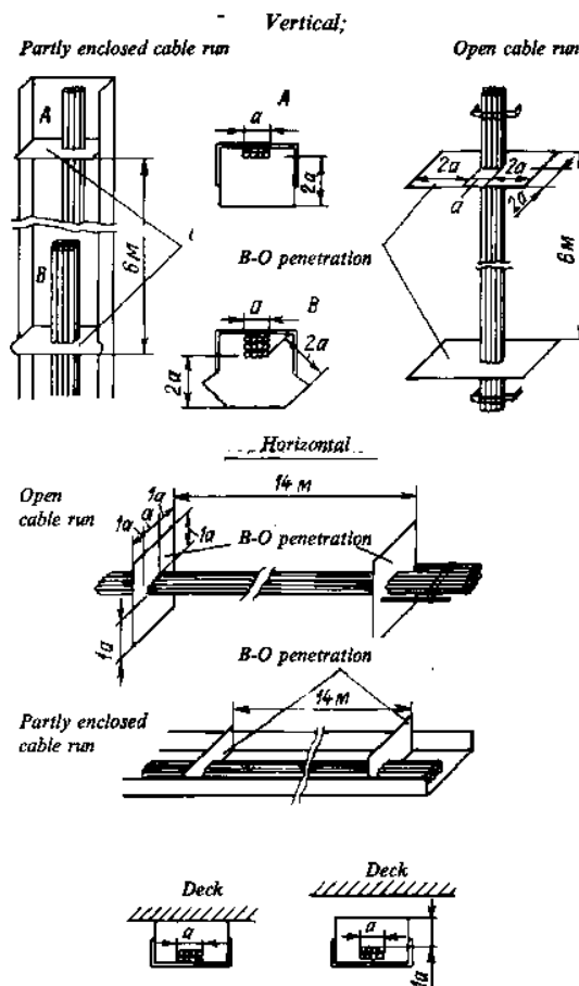
Fig. 16.8.4.3.2-2 Cable runs protection with B-O fire-retarding divisions
