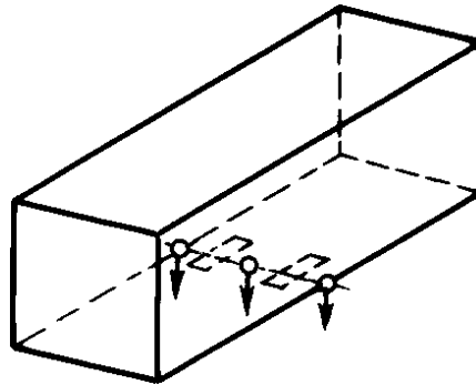
Fig. 3.9.1 Floor strength test
