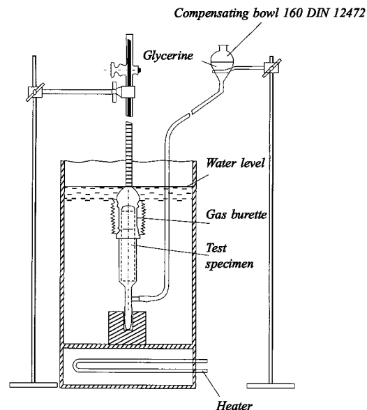
Fig. 5.4.6.9.1-1 Device for determination of the diffusible hydrogen content
