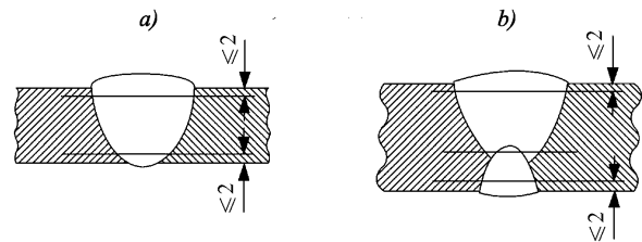
Fig. 6.4.4.5-1 Examples of hardness test with rows of indentations in butt welds:
