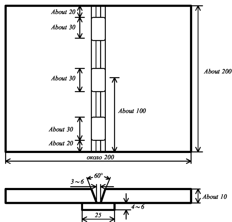
Fig. 9 Test piece P 1tack for tack butt welds
