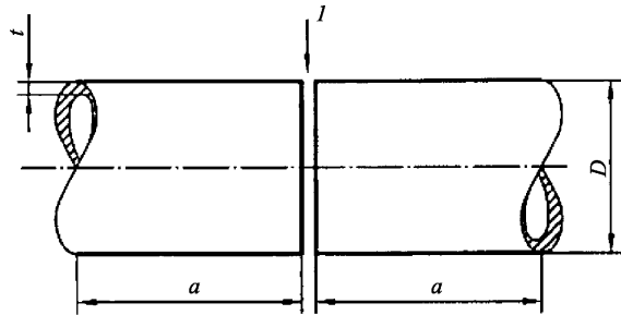
Fig. 8.2.2.5 Test piece for a butt joint in pipe: l — edge preparation and fit-up as detailed in pWPS; t — base metal thickness; a \geq 150 mm; D — outside pipe diameter
