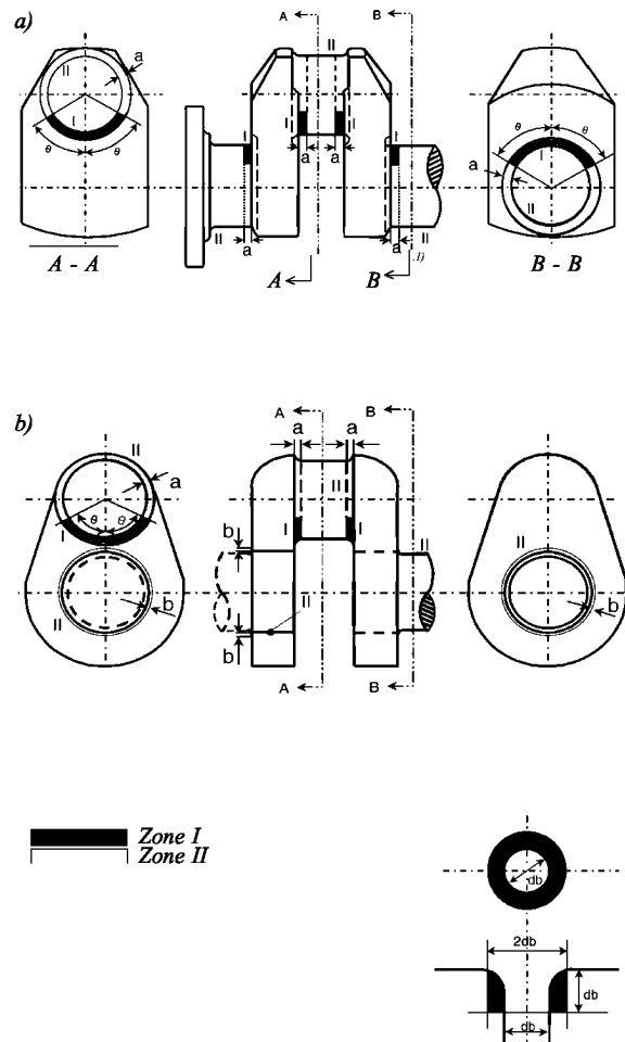
Fig. 2.5.2.3.3-1 Zones for magnetic particle/dye penetrant testing on crankshafts:
