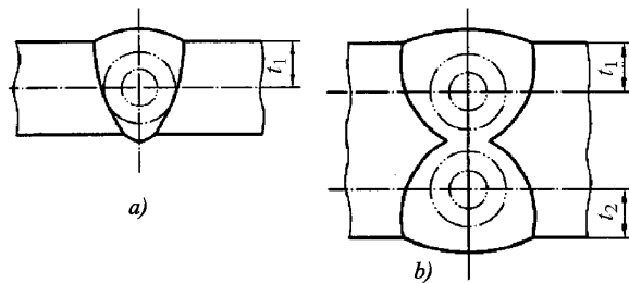
Fig. 6.4.4.1-5 Location of longitudinal round test specimens for tensile tests:
