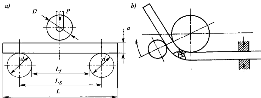
Fig. 6.4.4.2-2 Bend test methods:
