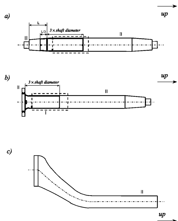
Fig. 2.5.2.3.3-4 Zones for magnetic particle/dye penetrant testing on rudder stocks:
