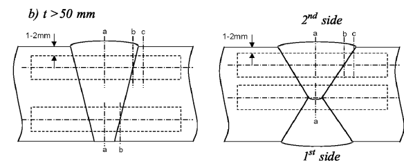
Fig. 6.4.4.4-2 Location of V-notch for butt weld of normal heat input (heat input \leq 50 kJ/cm):
