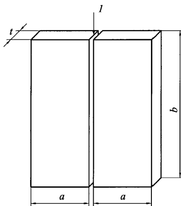
Fig. 8.2.2.4 Test piece for a butt joint in plate: l — edge preparation and fit-up as detailed in pWPS; t — base metal thickness; a \geq 150 mm (transverse bend test specimens may require a larger a ); b \geq 350 mm
