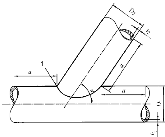
Fig. 6.3.1.6 Test piece for a branch connection: a \geq 150 mm;
