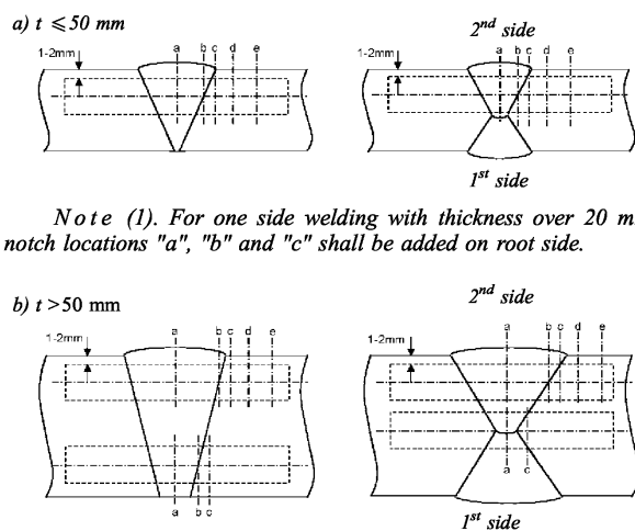
Fig. 6.4.4.4-3 Location of V-notch for butt weld of high heat input (heat input > 50 kJ/cm):
