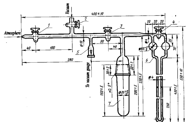
Fig. 5.4.6.8.1 Measuring device for determination of diffusible hydrogen content (GOST 23338-91, method 2):
