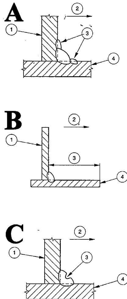
Fig. 5.4.5.3-2 Alternative methods for facilitating fillet weld fracture.
