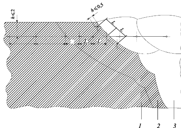
Fig. 6.4.4.5-2 Example showing the position of the indentations for hardness test in butt welds:
