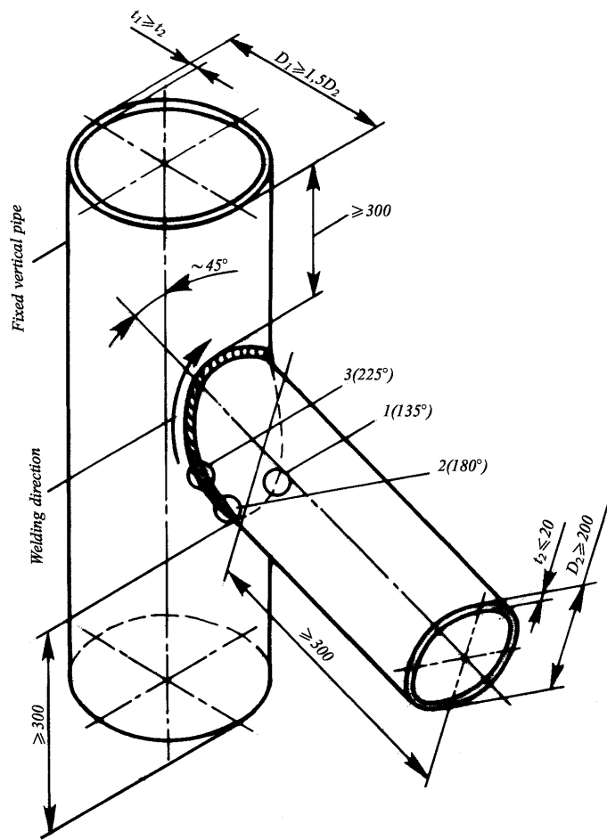
Fig. 7 Test piece for P 7 branch connection 1, 2, 3 — places of taking macrosections
