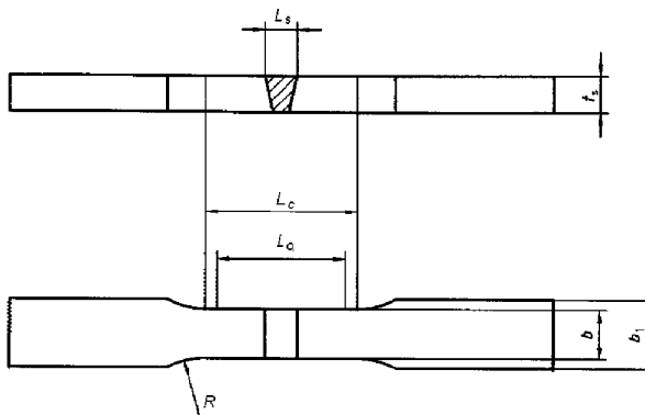
Fig. 6.4.4.1-1 Transverse specimen for tensile test of plates: L_s — greatest weld width (weld top); L_c = L_s + 60 mm — parallel test length; L_0 — gauge length; b — width of the parallel test length is defined as follows: b = 12 mm for t_s \leq 2 mm and b = 25 mm for t_s > 2 mm; b_1 \geq (b + 12) mm — width of the specimen gripping part; t_s — thickness of specimen; R \geq 25 mm — transition radius
