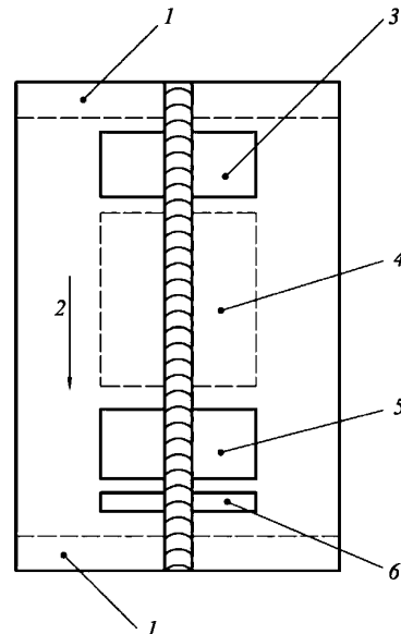
Fig. 8.3.2.1-1 Location of test specimens for a butt joint in plate:
