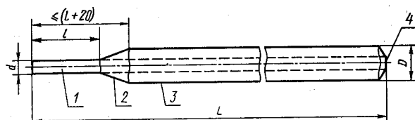
Fig. 5.3.3.2.3 Diagram for determination of the electrode nominal dimensions
