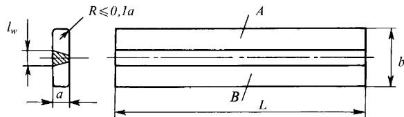
Fig. 6.4.4.2-3 Longitudinal bend test specimen for dissimilar welded joints:
