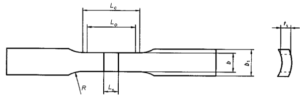
Fig. 6.4.4.1-2 Transverse specimen from a butt joint in pipes for tensile test:
