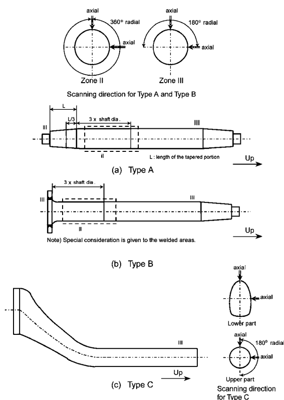
Fig. 2.5.2.4.3.1 Zones for ultrasonic testing on rudder stocks
