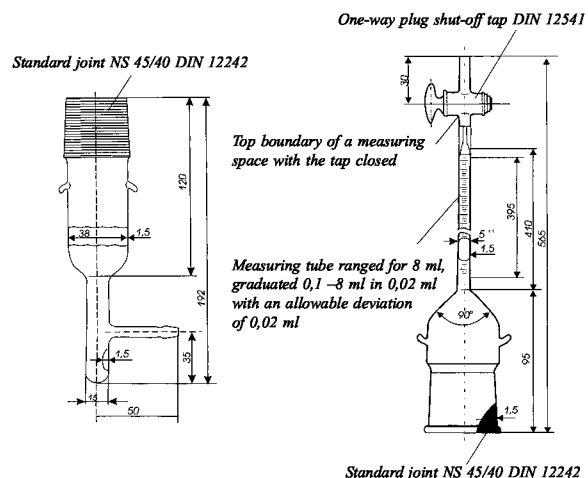
Fig. 5.4.6.6.1-2 Gas burette for determination of the diffusible hydrogen content
