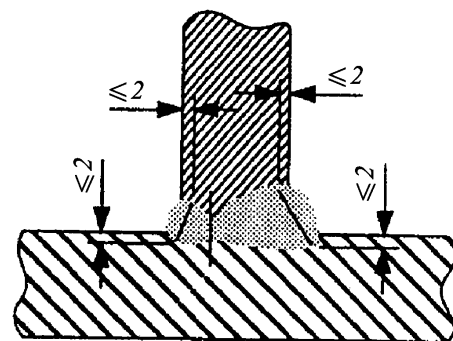
Fig. 6.4.4.5-3 Examples of hardness test with row indentation in T-joint welds with full penetration
