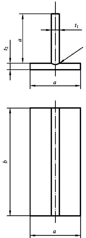
Fig. 8.2.2.6 Test piece for a tee-joint in plate and semi-finished product: l — edge preparation and fit-up as detailed in pWPS; t — base metal thickness; a \geq 150 mm; b \geq 350 mm
