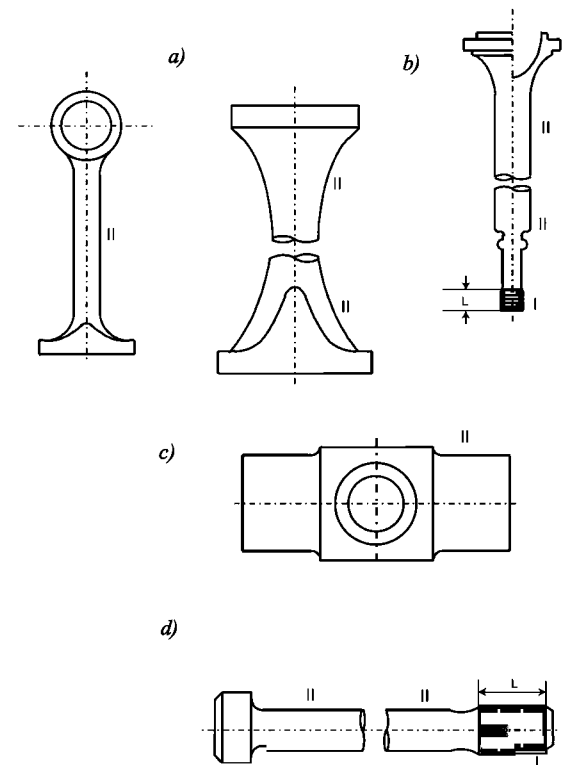
Fig. 2.5.2.3.3-3 Zones for magnetic particle/dye penetrant testing on machinery components:
