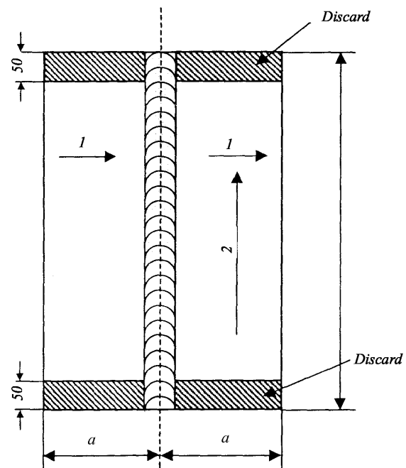
Fig. 6.3.1.2 Test piece for a butt-welded joint in plates: 1 – rolling direction for plates impact tested in the longitudinal direction KV_L (longitudinal specimens); 2 – rolling direction for plates impact tested in the transverse direction KV_T (transverse specimens); a and b – test piece dimensions adopted depending on a welding process: a \geq 150 mm, but not less than 3t and b \geq 350 mm, but not less than 6t for manual and semi-automatic welding; a \geq 200 mm and b \geq 1000 mm for automatic welding; t – thickness of the test piece
