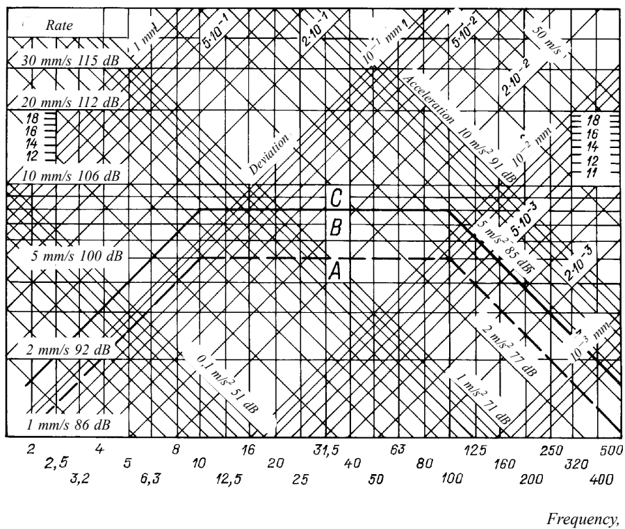
Fig. 9.5.2 Vibration standards for centrifugal separators:
