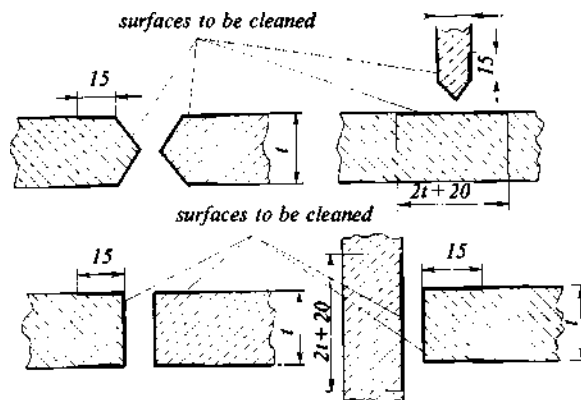
Fig. 2.8.10 Diagram of cleaning of edges in parts to be joined
