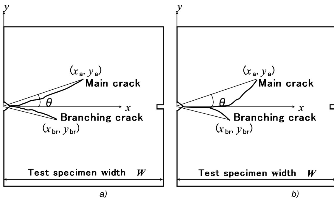
Fig. 2.2.11.1.6.4.2.2 Measurement methods of main crack and branch crack lengths: a — Case of branching from notch; b — Case of branching during brittle crack propagation
