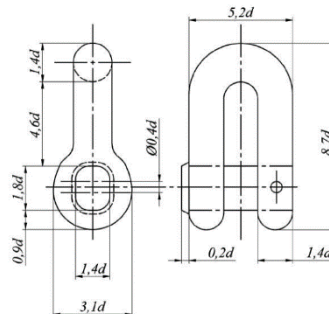
Fig. 7.1.3-6 End shackle
