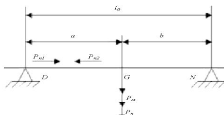
Fig. 4 Diagram of rotor loads during mechanical tests
