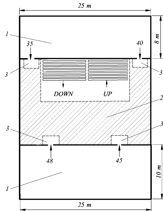
Fig. 7 Occupant loading calculation example:
