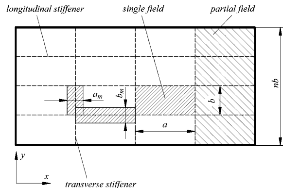
Fig. 7.10.6.24 General arrangement of panel
