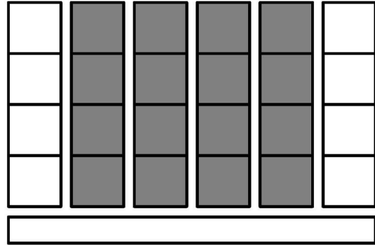
Fig. 7.10.6.12 Partial loading of a container hatch cover
