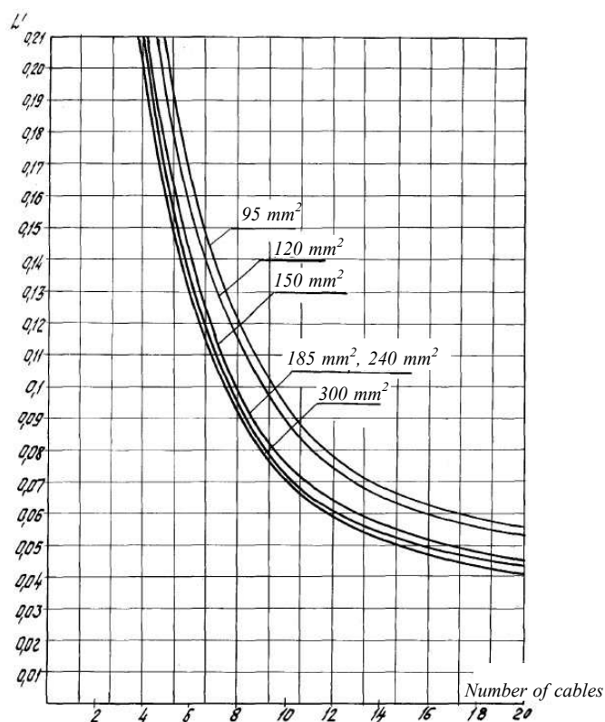
Fig. 8.6-2 Curves to determine the specific inductance of the cable run as function of the number of cables and cross-section of a conductor of cable of type "KHP", \text{H/m} \cdot 10^{-6}
