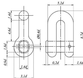
Fig. 7.1.3-6 End shackle
