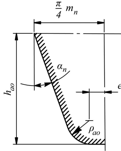
Fig. 4.2.2.7.3.2-2 Non-protuberance hob
