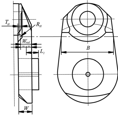
Fig. 2.4.6.1-2 Crank dimensions without web overlap necessary for calculation of stress concentration factors at T_H > R_H : W_{red} = design thickness of web, mm; W_{red} = W - T_H + R_H
