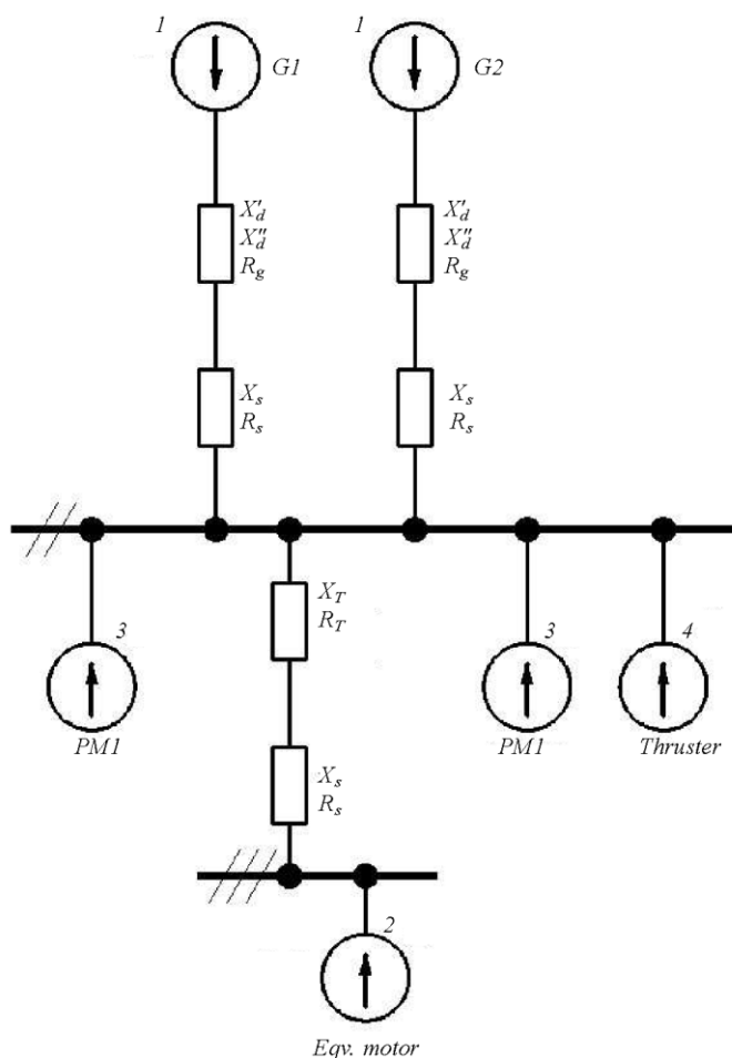
Design equivalent circuit of a PS with full distribution of the generated d.c. power, with asynchronous propulsion motors:
