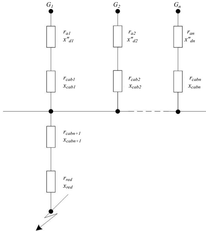
Fig. 8.2.1-1 The equivalent circuit for calculation of the SC current for generators in PS with partial d.c. power distribution:
