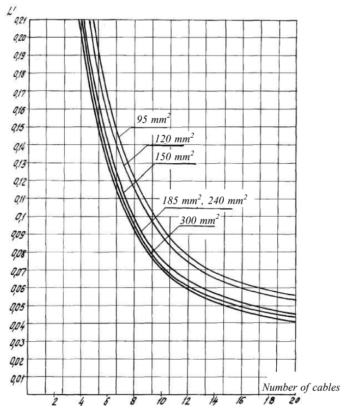
Fig. 8.6-2 Curves to determine the specific inductance of the cable run as function of the number of cables and cross-section of a conductor of cable of type "KHP", H/m \cdot 10^{-6}
