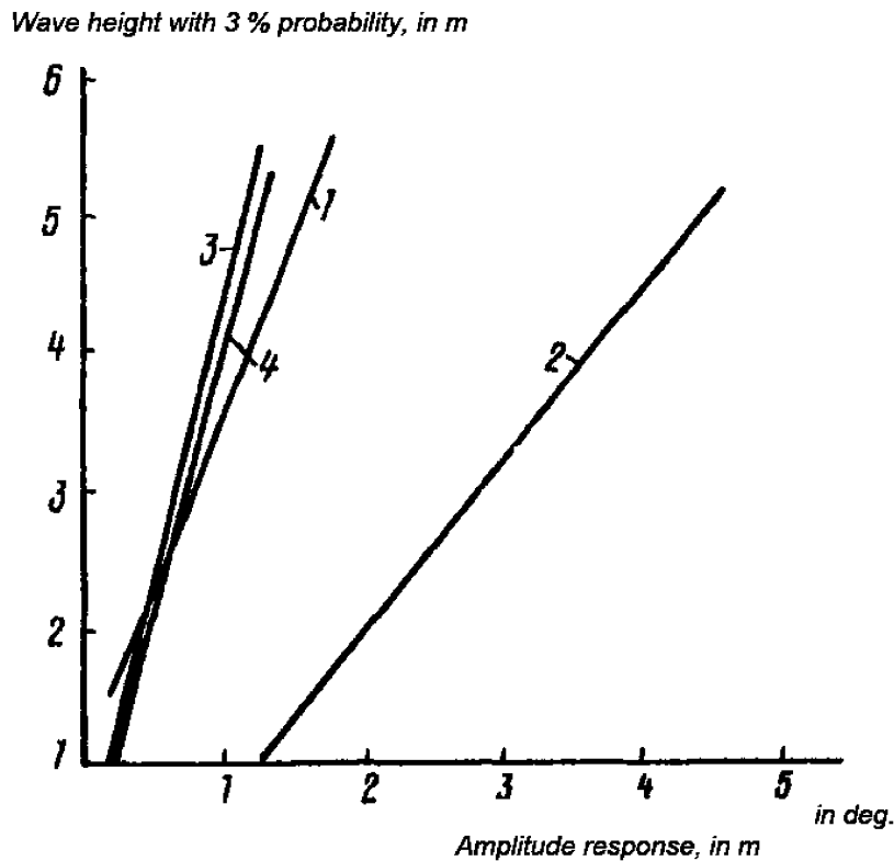
Fig. 7.3-1 Motion amplitudes of SULEYMAN VEZIROV in irregular waves with 3 % probability [2]: 1, 2 — pitch ( \psi ) and roll ( \theta ); 3, 4 — sway ( a_y ) and heave ( a_z )
