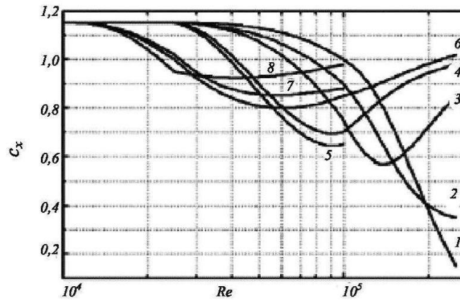
Fig. 4.3.1-3 Diagram of dependence of factor c_x on Reynolds number and relative roughness k of pipeline surface: 1 — k = 0 ; 2 — k = 5,0 \cdot 10^{-4} ; 3 — k = 2,0 \cdot 10^{-4} ; 4 — k = 4,0 \cdot 10^{-3} ; 5 — k = 5,0 \cdot 10^{-3} ; 6 — k = 7,0 \cdot 10^{-3} ; 7 — k = 9,0 \cdot 10^{-3} ; 8 — k = 2,0 \cdot 10^{-2}
