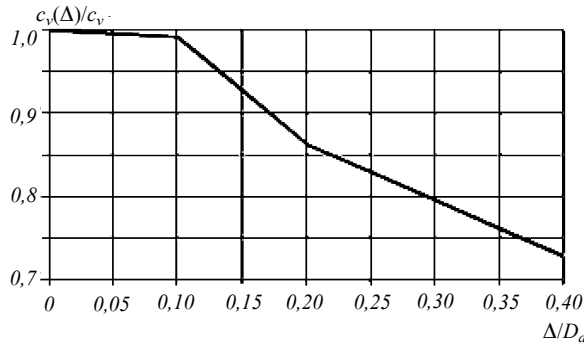
Fig. 7 c_v(\Delta)/c_v factor in relation to the relative pipeline burial \Delta/D_a
