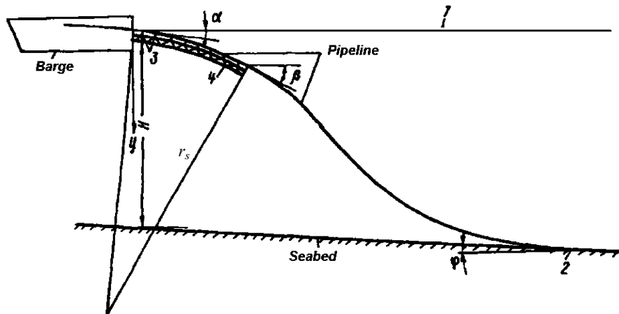
Fig. 7.2-1 Geometrical parameters of pipeline laying by S -method:
