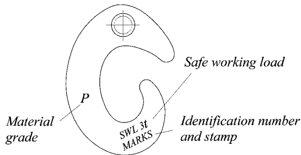
Fig. 11.2.1-1 Marking of hooks
