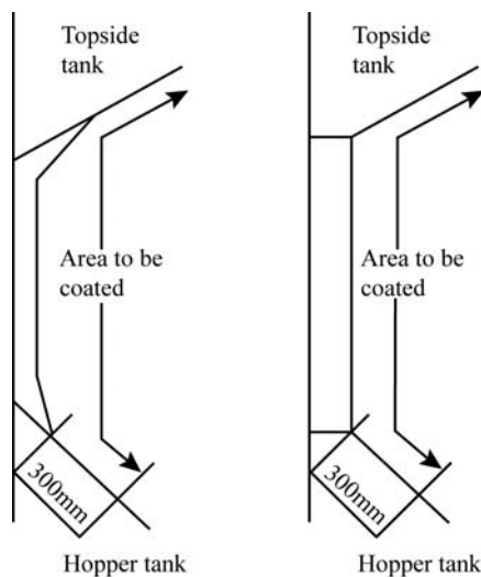
Figure 1: Side areas to be coated
