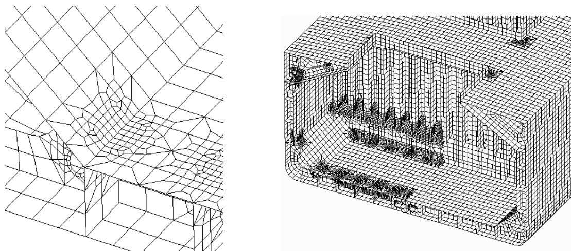
Figure 1: “Direct” modelling with refined meshes
