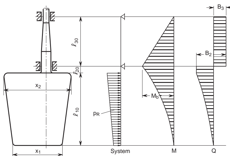
Figure 5: Semi-spade rudder (with 2-conjugate elastic supports)
