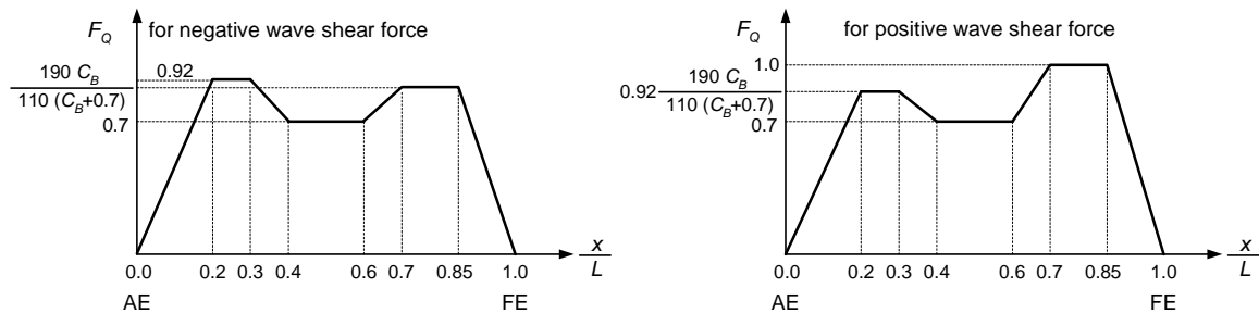
Figure 4: Distribution factor F_Q
