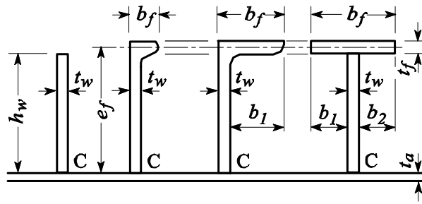
Figure 2: Dimensions of stiffeners
