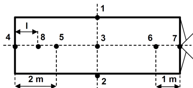
Fig. 3.9.3 Places for measuring deformations l = 0,7 \dots 1,2 m
