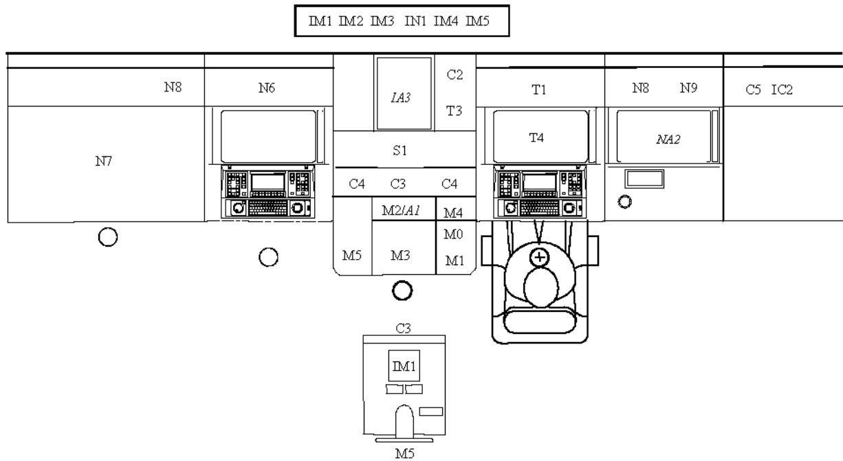
Redundant workstations
