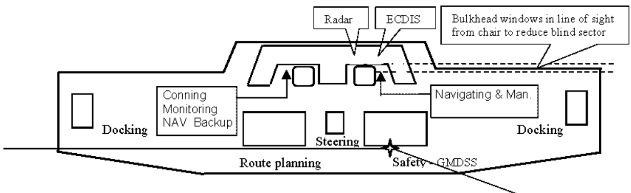
Fig. 2.5.17-2 Required field of vision from the radio station when to be controlled and infrequently used for short periods of time by the watch officer. Navigation based on electronic chart system (ECDIS) – Conning position at console
