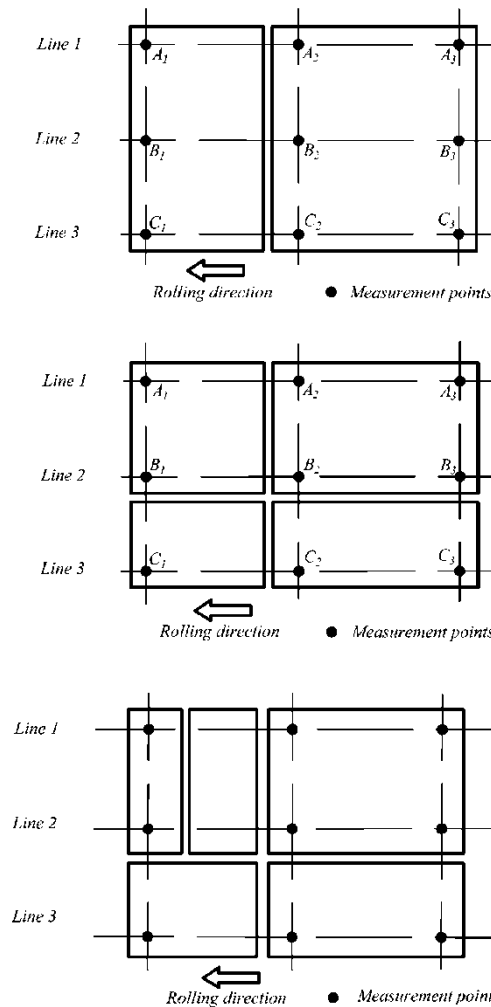
Fig. 3.2.8.5.1-2 Locations of thickness measuring points for the cut steel products
