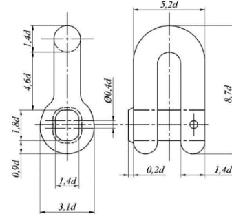
Fig. 7.1.3-6 End shackle
