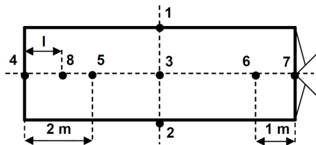
Fig. 3.9.3 Places for measuring deformations l = 0,7 \dots 1,2 \text{ m}
