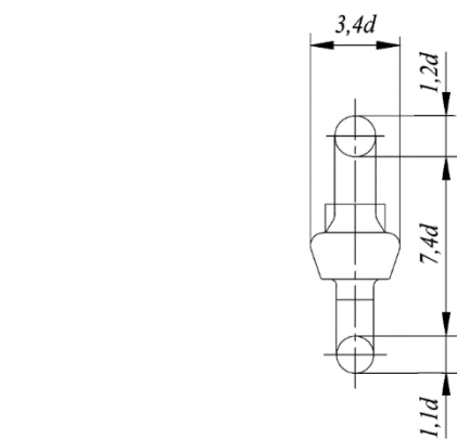
Fig. 7.1.3-5 Joining shackle
