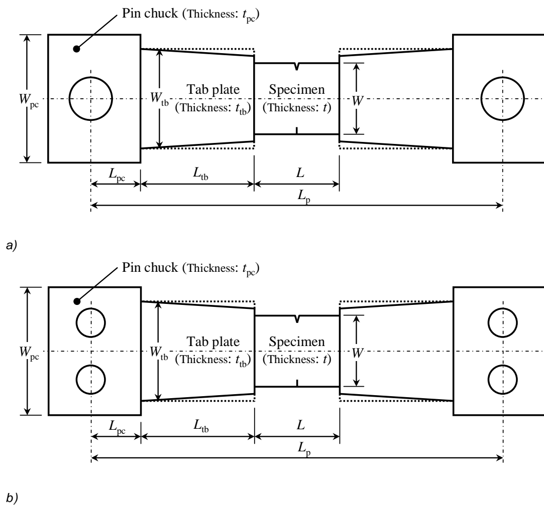
Fig. 2.2.11.1.4.2-1 Definitions of the dimensions of the tab plates and pin chucks: a) — Single-pin type; b) — Double-pin type
