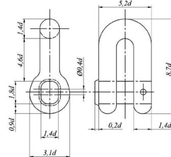
Fig. 7.1.3-6 End shackle
