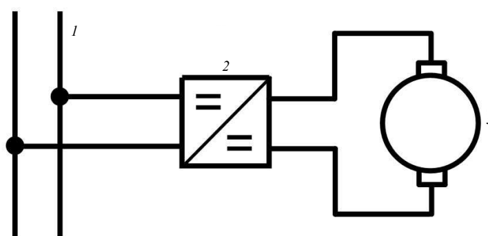
Fig. 3.3.2 Connection diagram of a d.c. electric drive to the d.c. main switchboard: 1 – d.c. main switchboard; 2 – semiconductor d.c.-d.c. converter; 3 – d.c. electric motor
