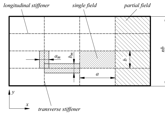
Fig. 7.10.6.24 General arrangement of panel
