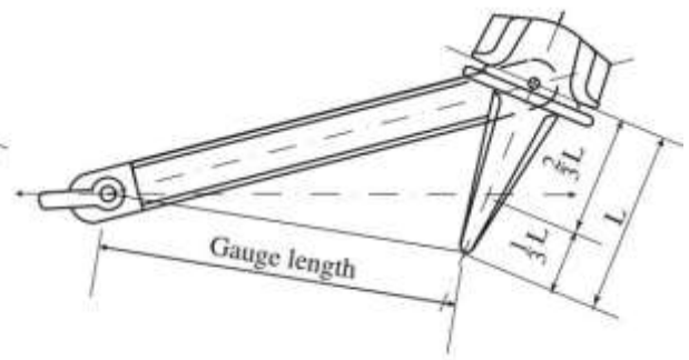
Stocked Anchor
