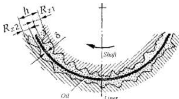
Fig. 3 Lubricating oil layer for a steady-state operating condition
