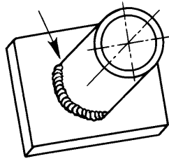
PA: Flat position Pipe: rotating Axis: inclined
