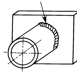
PB: Horizontal-vertical position Pipe: rotating Axis: horizontal
