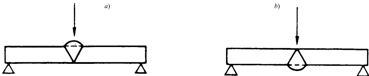
Fig. 4.4.4.2-2 Diagram of the fracture testing root-bend test (a) and fracture testing face-bend test (b) of the test specimens from the test piece P_1 of the butt plate joint
