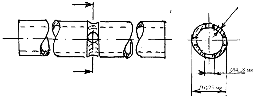
Fig. 4.4.4.4-3 Tension test specimen with 4 holes for testing butt joints of small diameter pipes
