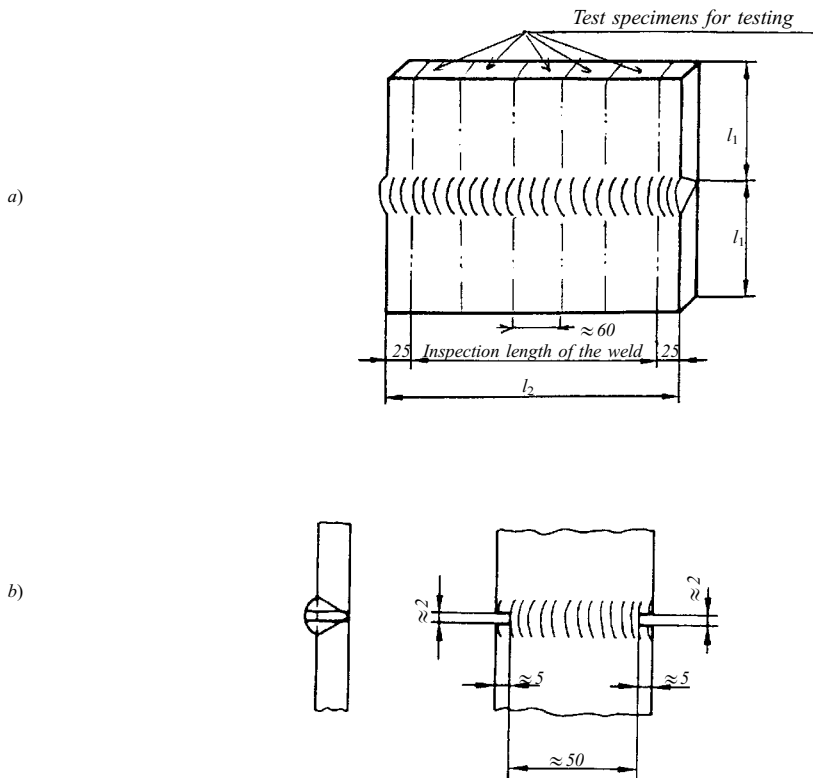
Fig. 4.4.4.2-1 Diagram of cutting-out (a) and test specimens from the test piece P_1 of the butt plate joint for weld metal fracture testing (b)
