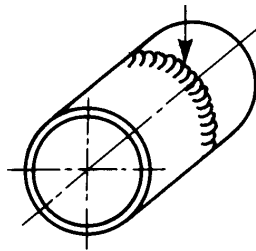
PA: Flat position Pipe: rotating Axis: horizontal
