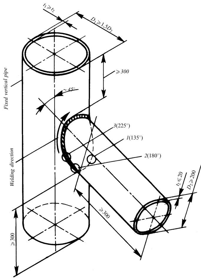
Test piece of P 7 pipe joint unit 1, 2, 3 = place of taking macrosections
