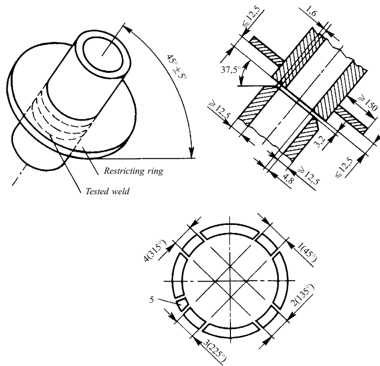
Test piece of P 6 pipe joint with a restricting rings: 1, 2, 3, 4 = places for taking test specimens for static bend; 5 = place for taking a macrosection
