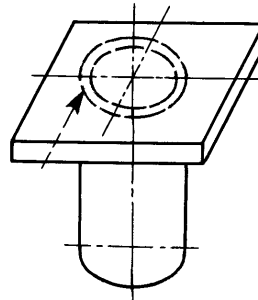
PC: Horizontal overhead position Pipe: fixed Axis: vertical
