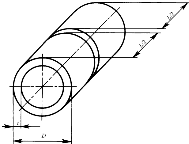
Test piece of P 3 butt joint in pipes
