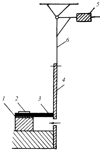
Fig. 2 Diagram of a test unit 1 = input lead; 2 = holder with clamps; 3 = filament loop; 4 = sample; 5 = mass; 6 = frame with a sample holder
