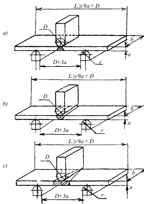
Fig. 4.4.4.2-3 Dimensions of test specimens from the test pieces of the butt plate joints ( P_1 ) and butt pipe joints ( P_3 , P_5 and P_6 ), and the diagram of the static face-bend test (a), root-bend test (b) and side-bend test (c)
