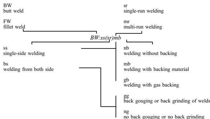
Fig. 4.3.3.2 Coding diagram for weld type and welding details
