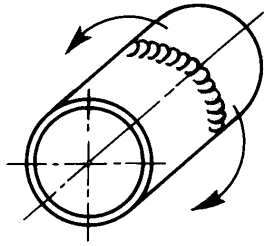
PG: Vertical downwards position Pipe: fixed Axis: horizontal
