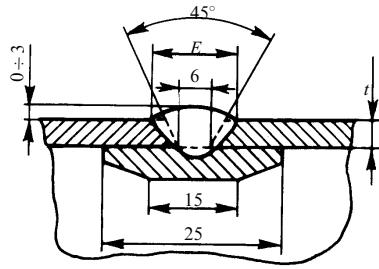
Details of edges and weld preparation:
