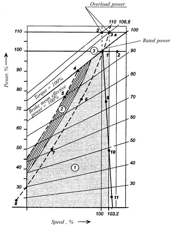
Fig. 3.1.1 Power/Speed Diagram:
