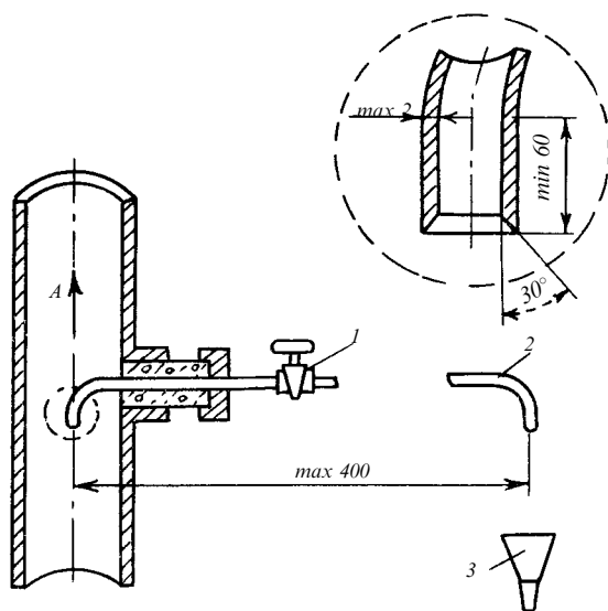
Fig. 2.7-1 Diagram of sampling arrangements: 1 – straight-through stopcock; 2 – 6 mm bore pipe; 3 – funnel to drainage; A – direction of flow
