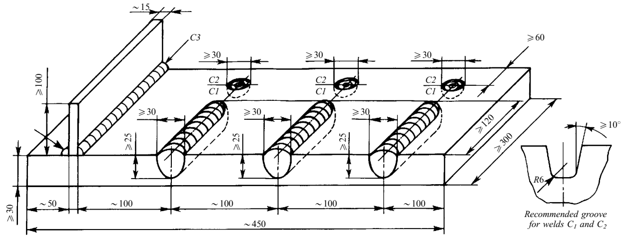
Test piece — simulator P 8 of castings and forgings repair
