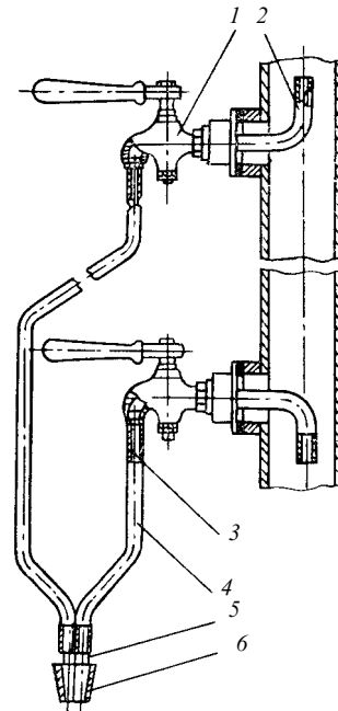
Fig. 2.7-2 Arrangement for taking samples from supply pipes: 1 – sampling cock; 2 – angular branch pipe; 3 – tip; 4 – hose; 5 – connection; 6 – plug
