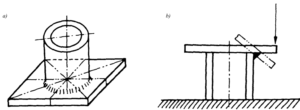
Fig. 4.4.4.5 Diagram of cutting-out (a) and fracture (b) testing of test specimens from pipe T-joint P 4 test pieces
