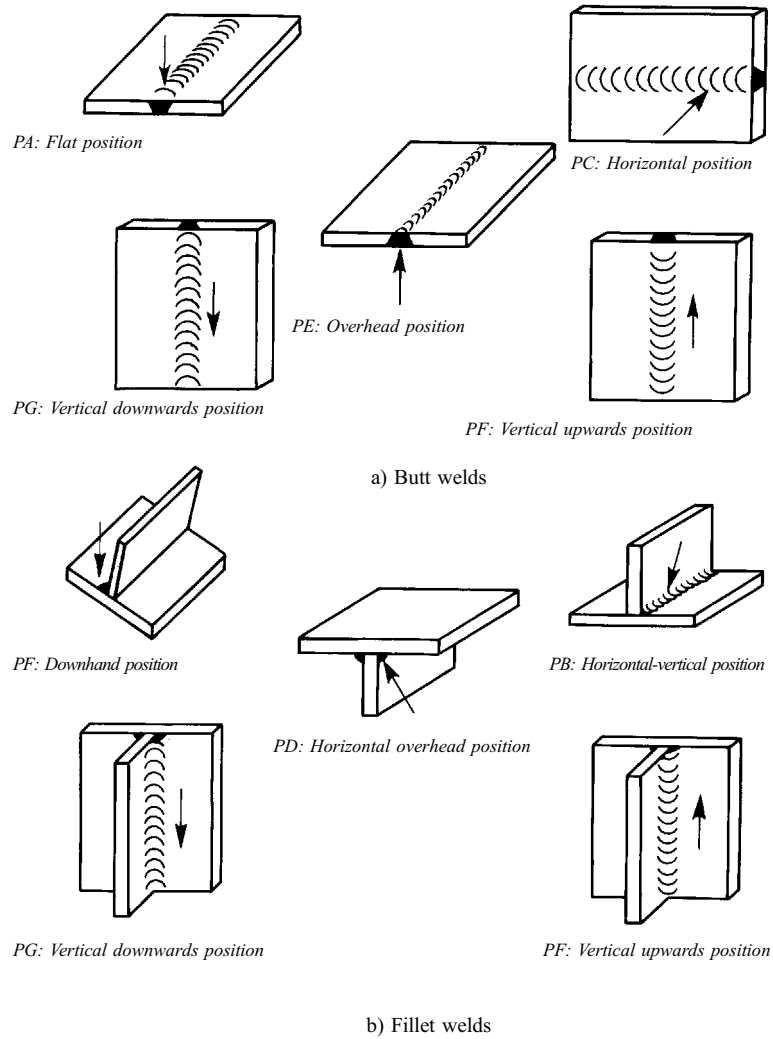
Fig. 1 Welding positions for plates
