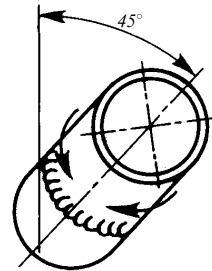
J-L045: Inclined downwards position Pipe: fixed Axis: inclined
