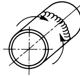
PF: vertical upwards position Pipe: fixed Axis: horizontal
