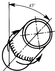
H-L045: Inclined upward position Pipe: fixed Axis: inclined
