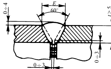
Test piece of pipe joint with a limited access to the welding zone P 5
