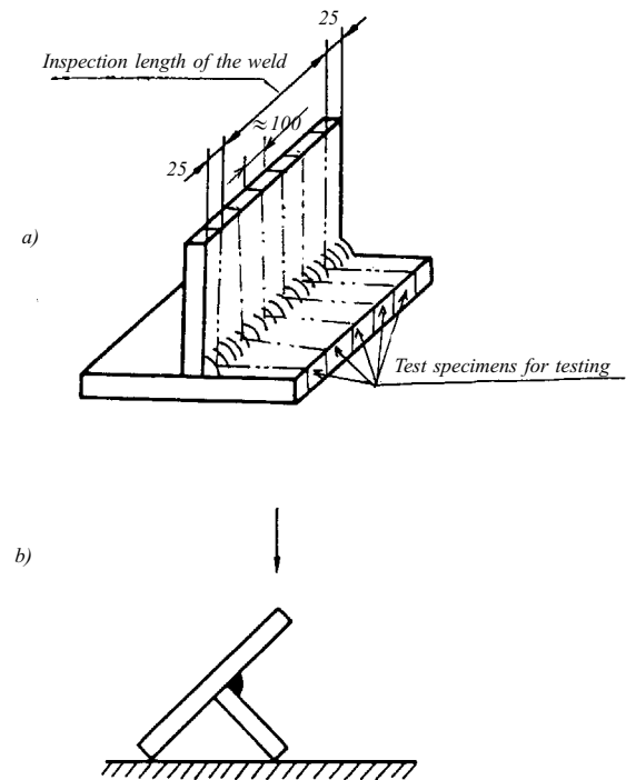
Fig. 4.4.4.3 Diagram of cutting-out (a) and test specimens from the test piece P_2 of the T-joint for weld metal fracture testing (b)
