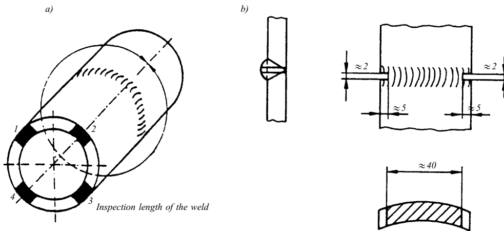
Fig. 4.4.4.4-1 Diagram of cutting-out (a) and test specimens from the test pieces P 3 , P 5 and P 6 of butt pipe joints (b) for weld metal fracture testing; 1, 2, 3 and 4 = places for the selection of static bend test specimens from the test pieces prepared using slag-free methods of welding.
