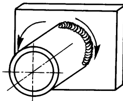
PC: Horizontal-vertical position Pipe: fixed Axis: horizontal
