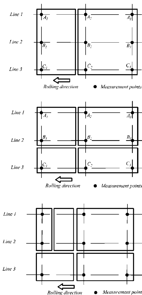
Fig. 3.2.8.5.1-2 Locations of thickness measuring points for the cut steel products
