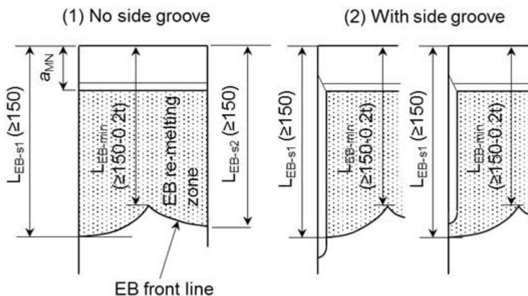
Fig. 2.2.11.4.4.5.2 Definition of EBW length
