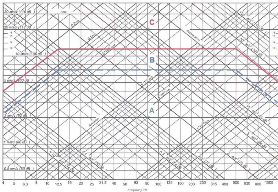
Fig. 9.9.3 Vibration standards of main azimuth thrusters
