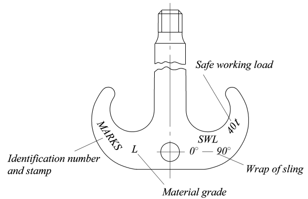
Fig. 11.2.1-2 Marking of ramshorn hooks
