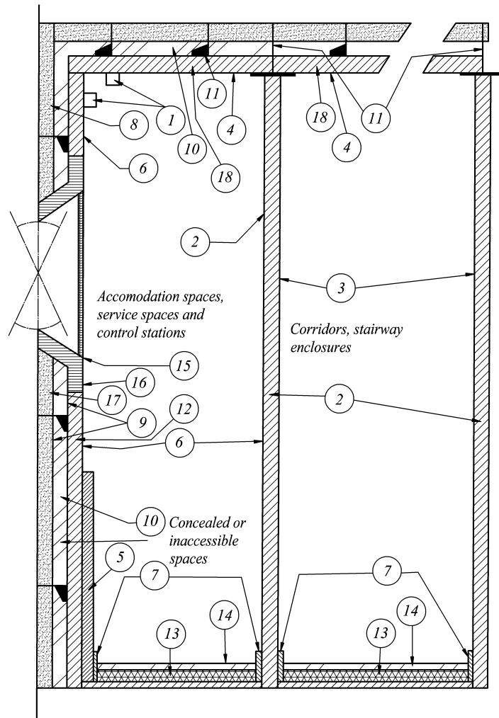
Fig. 2.3.10 Structural members
