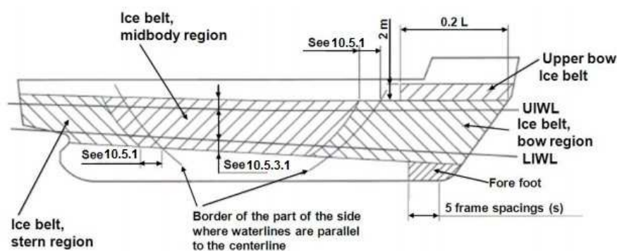
Fig. 10.5.1.1 Ice strengthened regions of the hull
