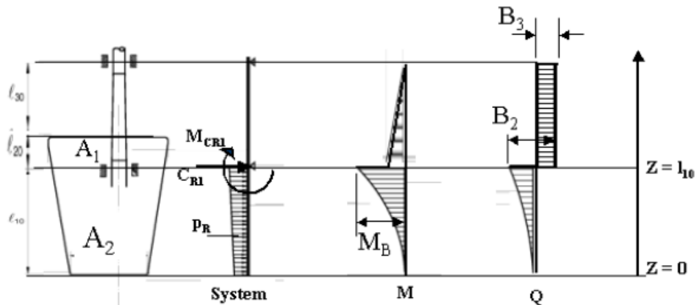
Figure 7: Spade rudders with rudder trunks
