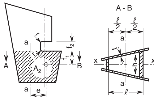
Figure 10: Geometry of rudder
