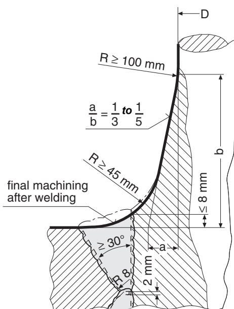
Figure 21: Welded joint between rudder stock and coupling flange
