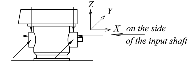
Fig. 9.9.2 Points of vibration measuring of azimuth thrusters
