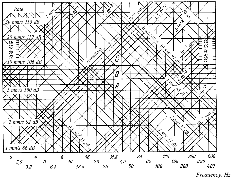
Fig. 9.7.1 Vibration standards for boilers, auxiliary machinery and equipment:
