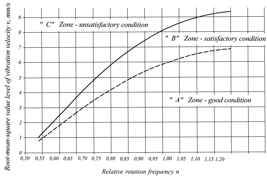
Fig. 9.9.3 Vibration standards of azimuth trusters
