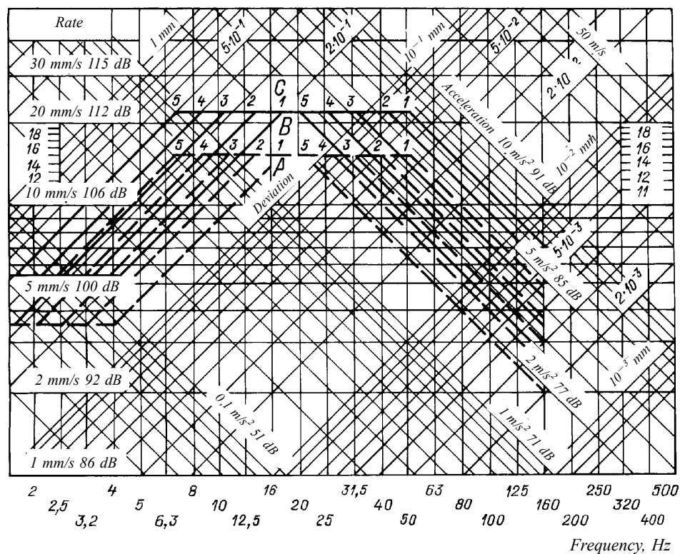
Fig. 9.3.2 Vibration standards for internal combustion engines with a piston stroke: 1 — under 30 cm; 2 — 30 to 70 cm; 3 — 71 to 140 cm; 4 — 141 to 240 cm; 5 — over 240 cm. ----- Upper limit of category A; ————— Upper limit of category B
