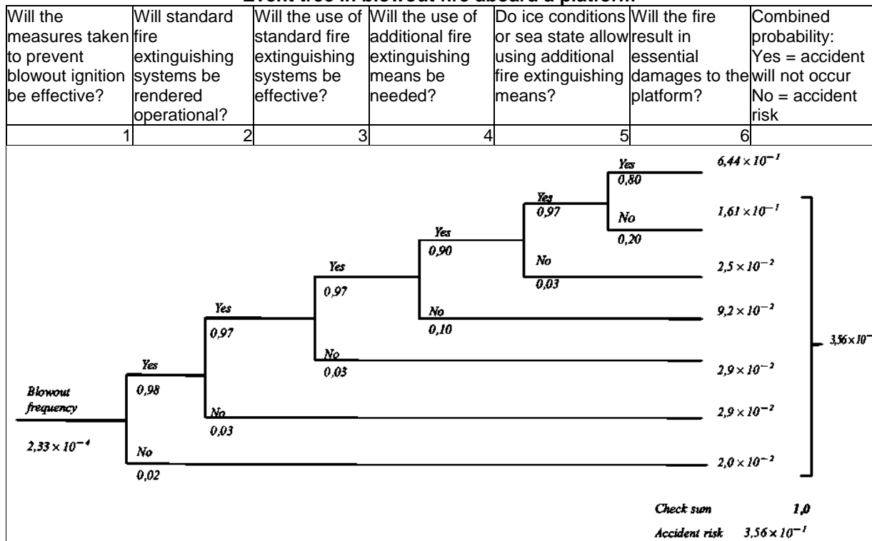
Event tree in blowout fire aboard a platform
