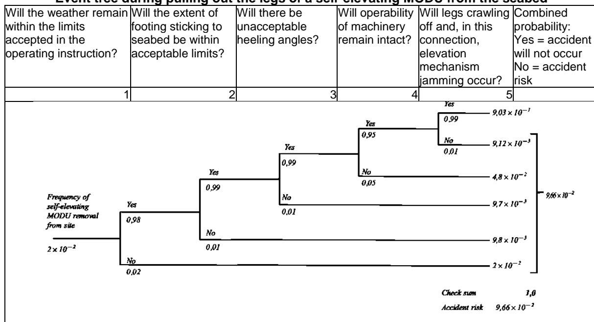
Event tree during pulling out the legs of a self-elevating MODU from the seabed
