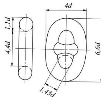
Fig. 7.1.3-2 Enlarged link
