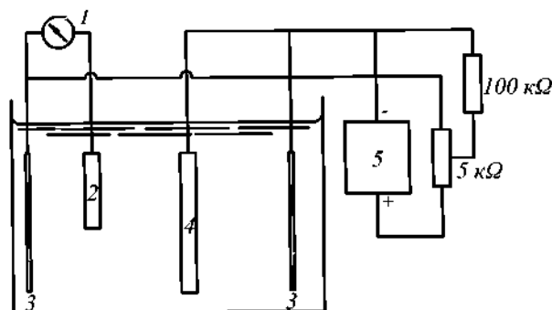
Fig. 2.5.6.1-2 Cathode protective circuit with galvanostatic control:
