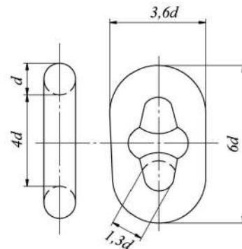
Fig. 7.1.3-1 Common link
