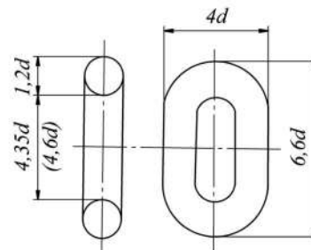
Fig. 7.1.3-3 Studless link
