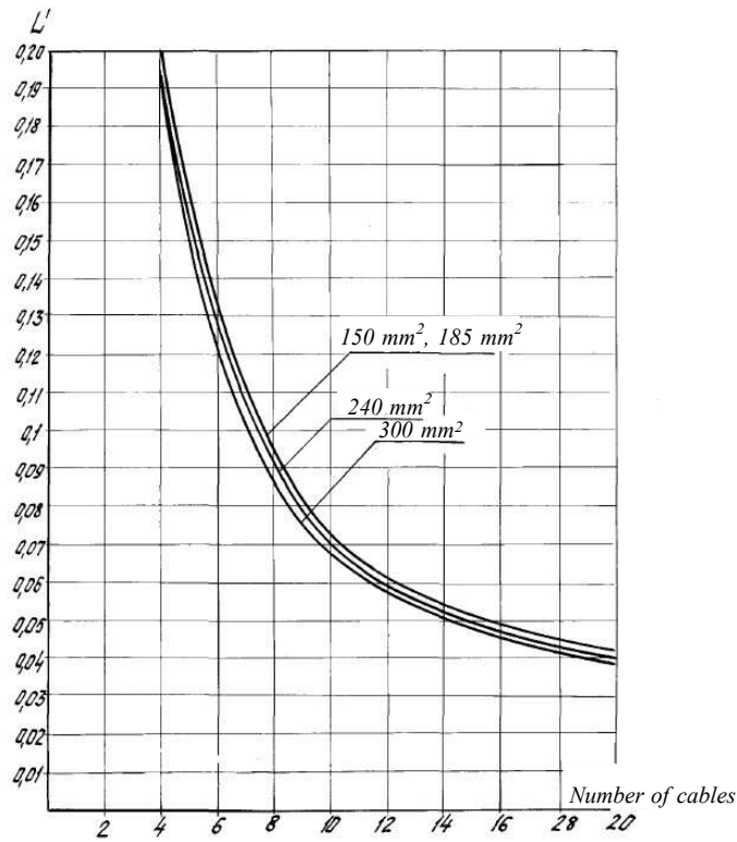
Fig. 8.6-3 Curves to determine the specific inductance of the cable run as function of the number of cables and cross-section of a conductor of cable of type "HPIIM", H/m • 10 -6
