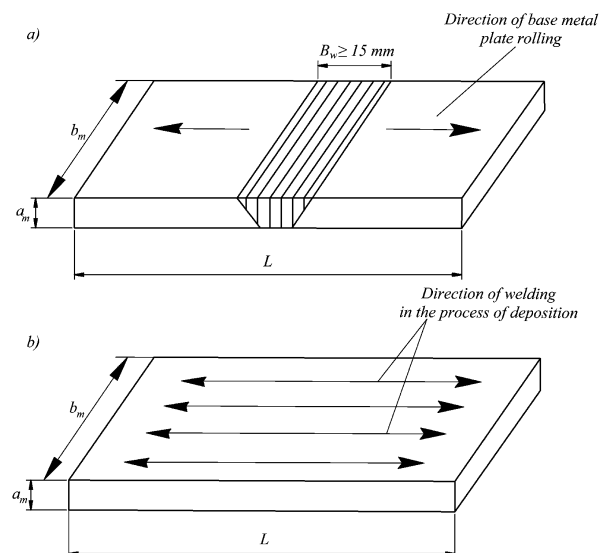
Fig. 4.8.4.3.2 Specimens for tests intended to define resistance to intercrystalline corrosion:
