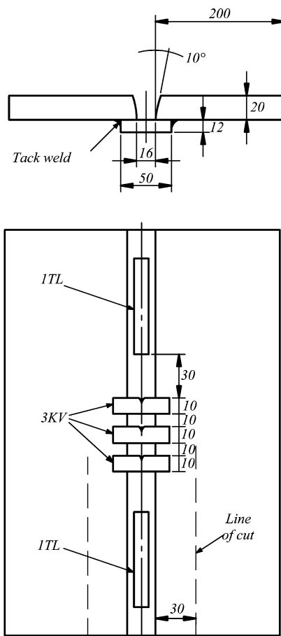
Fig. 4.4.2.2.1 Test assembly of deposited metal during testing of "wire — flux" combinations (test specimens are designated according to Table 4.4.1.4)
