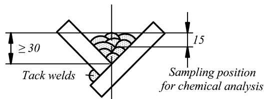
Fig. 4.10.2 Deposited metal test assembly
