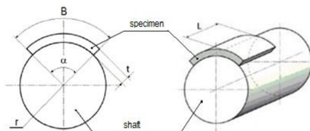
Fig. 6.13.3.3.1 Dimensions of testing specimen:
