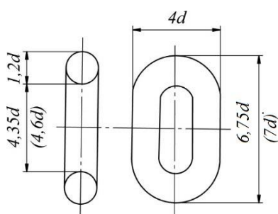
Fig. 7.1.3-3 Studless link
