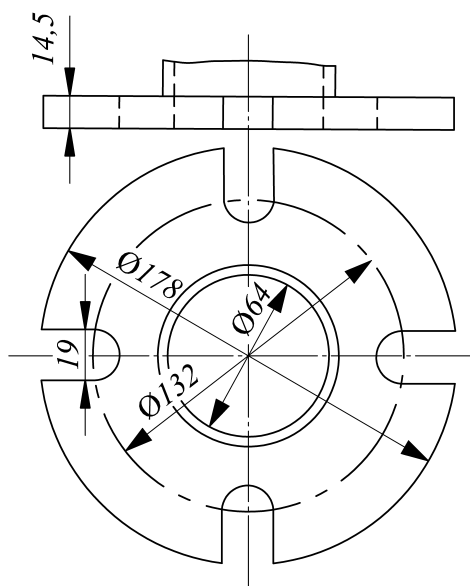
Fig. 5.1.18 International shore connection (ship)
