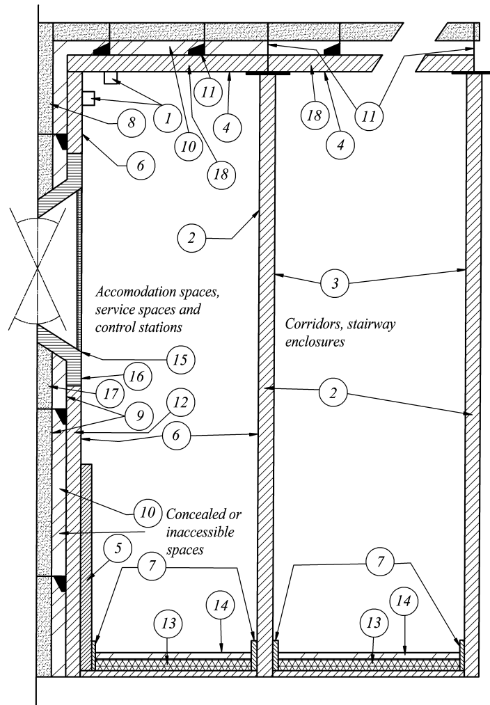
Fig. 2.3.10 Structural members
