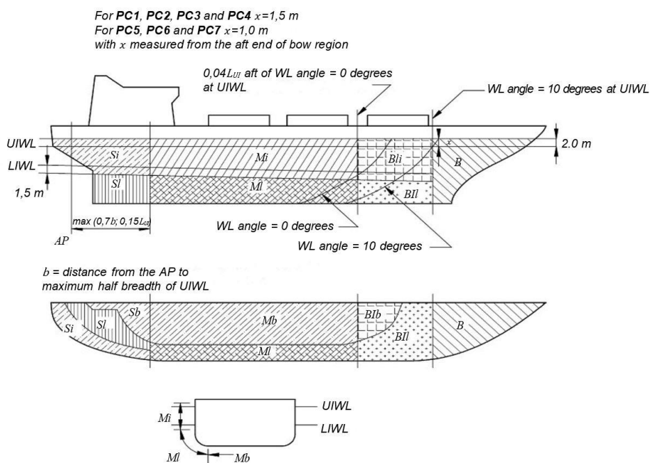
Fig. 1.2.2.1 Hull area extents
