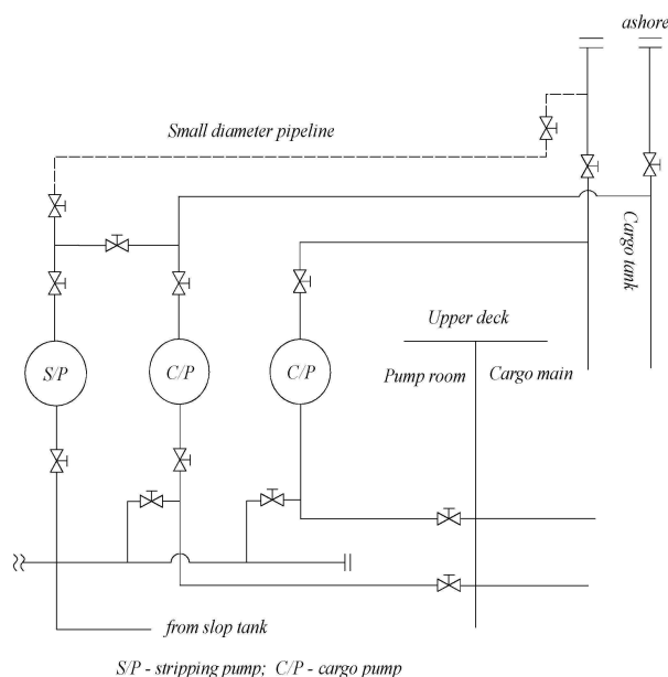
Fig. 9.12.9 Connection of the small diameter pipeline to the ship's manifold valvenaprybka
