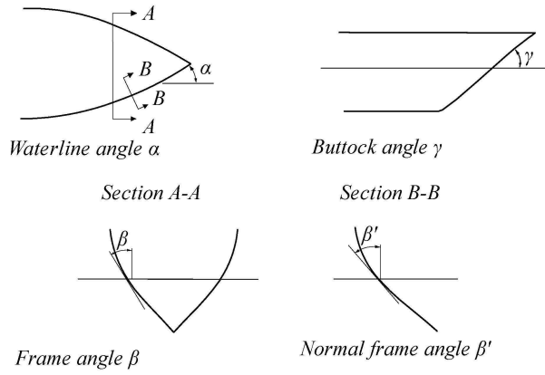
Fig. 1.2.3.2.1 Definition of hull angles
