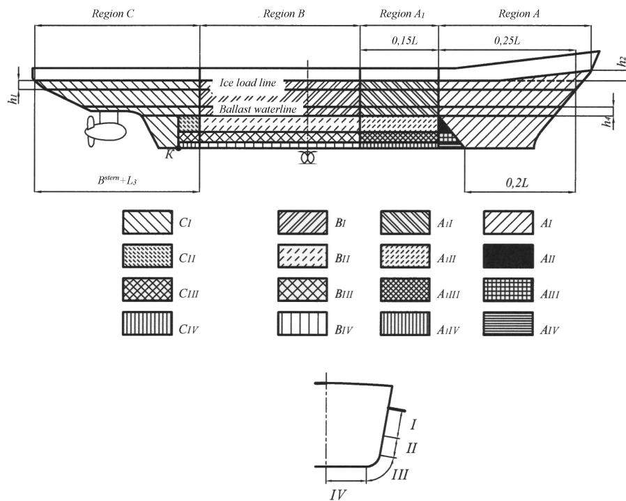
Fig. 19.2.2.3 Regions of ice strengthening of Arctic double acting ships with ice class mark Icebreaker6 or Icebreaker7 in the class notation when operating stern first: b^{stern} = distance from the point of the ice load line and sternframe intersection to the section where the ice load line is the widest, but not greater than 0,2L
