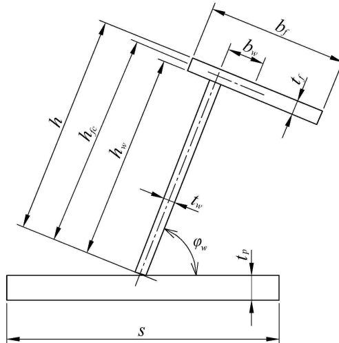
Fig. 1.2.5.7 Stiffener geometry
