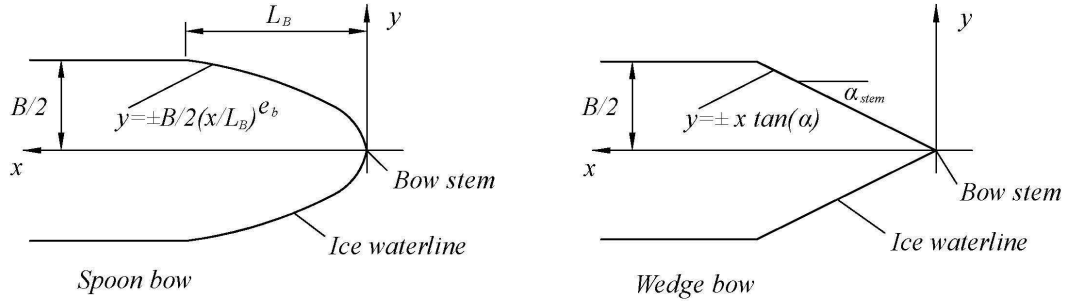
Fig. 1.2.13.2.1-1 Bow shape definition
