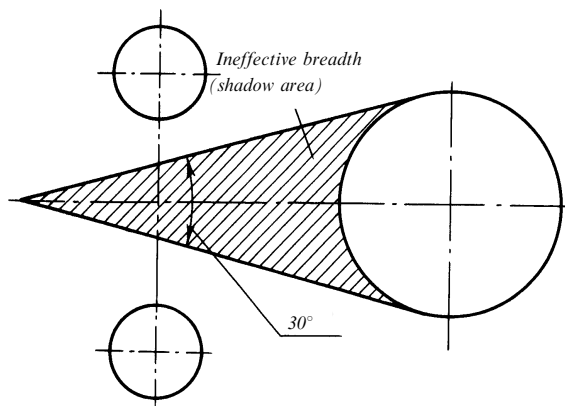
Fig. 1.4.8.3 Design section
