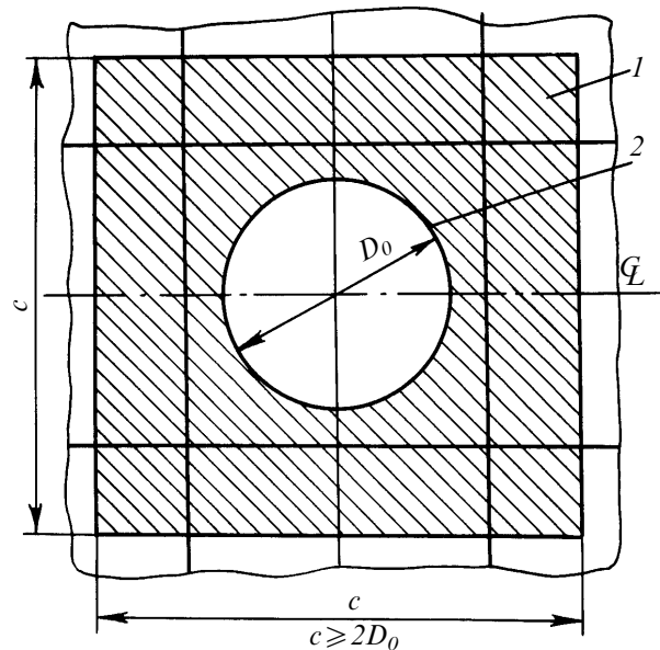
Fig. 3.6.4.12.5: I — thickened plate; 2 — tub
