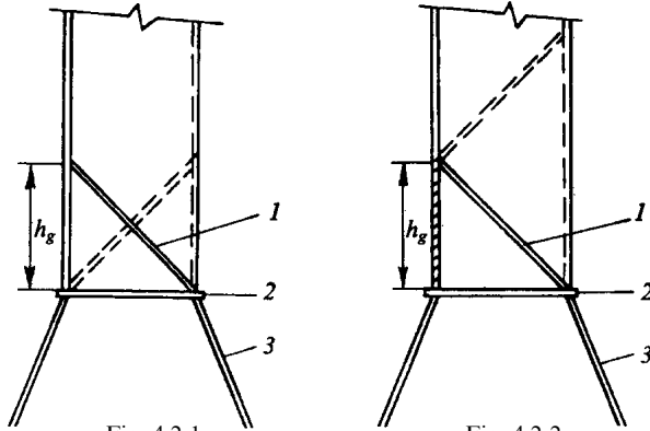
Fig. 4.2-1 Symmetrical shedder plates:
