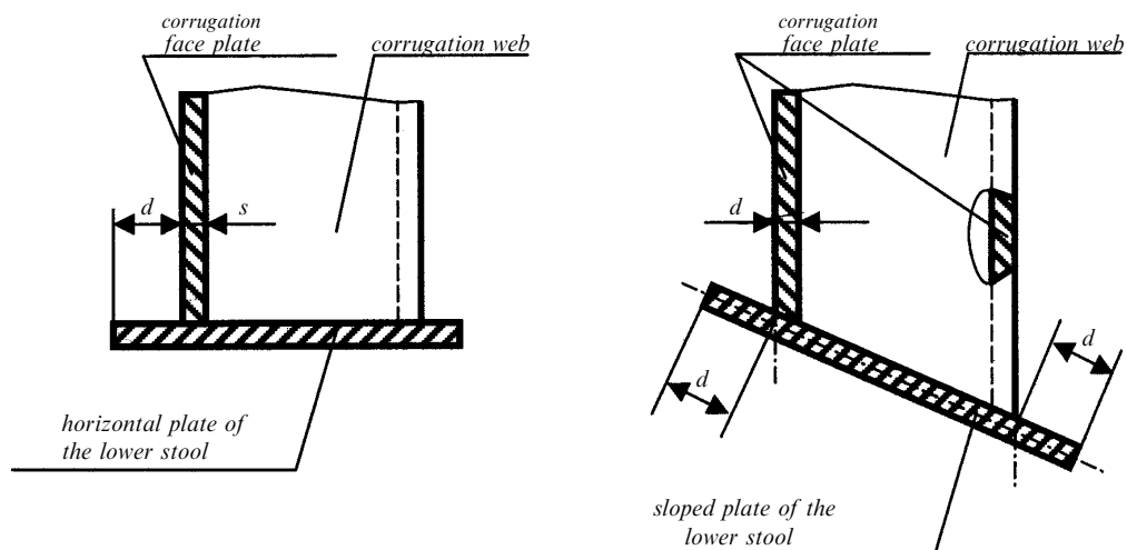
Fig. 4.1: s = as-built flange thickness; d \geq s
