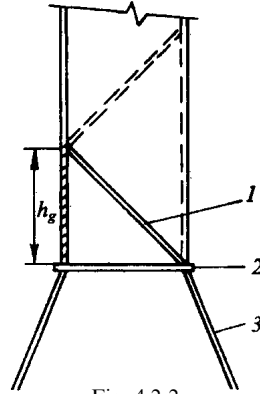
Fig. 4.2-2 Unsymmetrical shedder plates:
