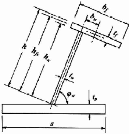
Fig. 1.2.5.7 Stiffener geometry
